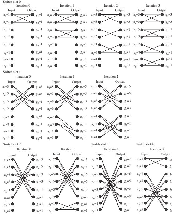
Fig. 6. Example of the number of iterations for k FRR to converge for an 8 \times 8 SDMG CIOQ switch under saturated load.
