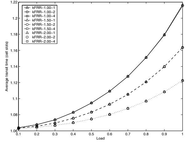
Fig. 7. Average transit time vs. load of k FRR with g = 1 , k = 2 and different number of iterations under Bernoulli arrivals.
