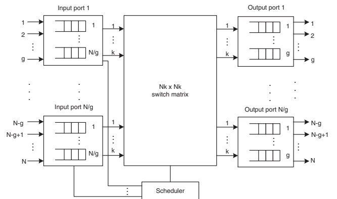
Fig. 2. An SDMG CIOQ switch.
