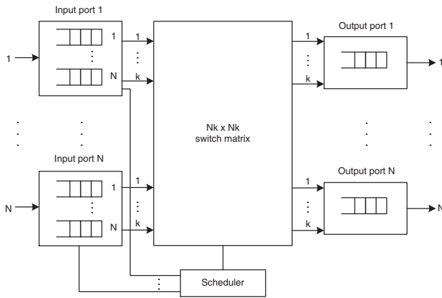
Fig. 3. An SDMGM CIOQ switch with g = 1 .
