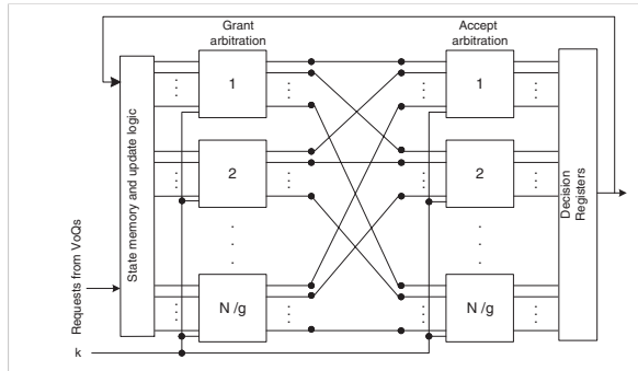
Fig. 13. Block diagram of a one-iteration k FRR scheduler for an N \times N SDMG CIOQ switch.
