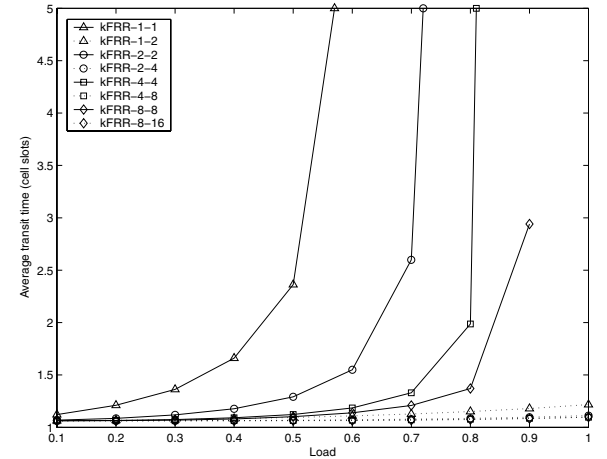
Fig. 8. Average transit time vs. load of one-iteration k FRR with different group factors and different port connection factors under uniform Bernoulli arrivals.
