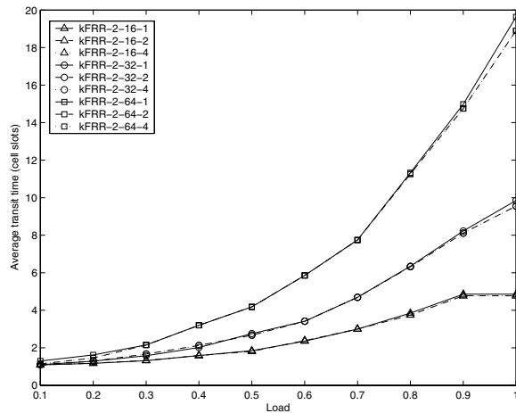
Fig. 10. Average transit time vs. load of k FRR with k = 2 , g = 1 and different number of iterations under bursty arrivals.
