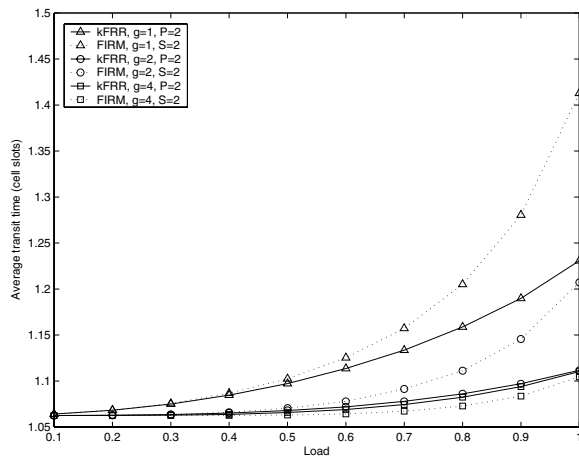
Fig. 9. Average transit time vs. load of one-iteration k FRR with P = 2 and one-iteration FIRM with S = 2 under uniform Bernoulli arrivals.
