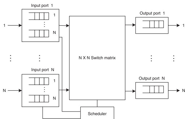
Fig. 1. A CIOQ switch.
