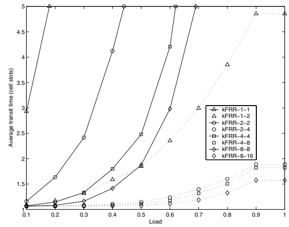
Fig. 11. Average transit time vs. load of one-iteration k FRR with different group factors and different port connection factors under bursty arrivals.
