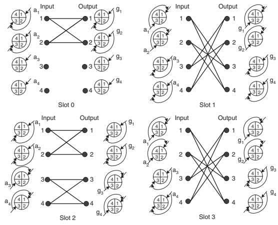
Fig. 5. Illustration of desynchronization effect of grant pointers of k FRR for a 4 \times 4 SDMG CIOQ switch under saturated load.
