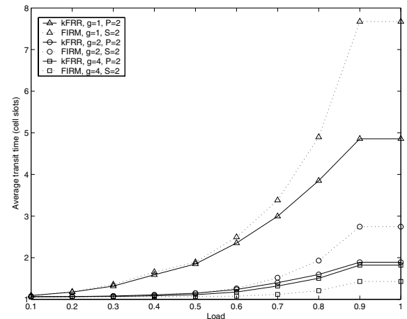
Fig. 12. Average transit time vs. load of one-iteration k FRR with P = 2 and one-iteration FIRM with S = 2 under bursty arrivals.
