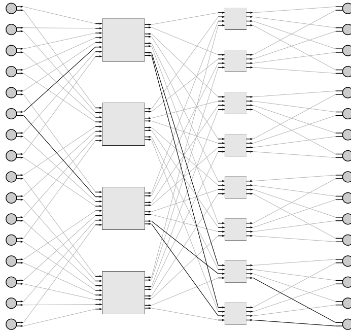
Figure 20.9 16 × 16 Square Multipath Network Constructed from RN1 Routing Components
