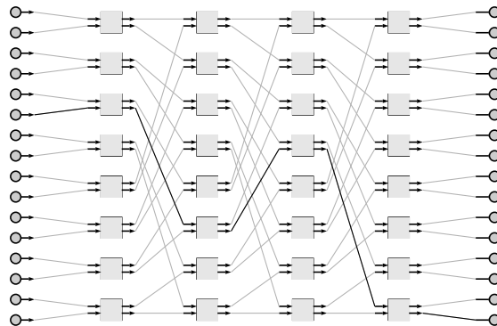
Figure 20.3 16 × 16 Square Multipath Network Constructed from 2 × 2 Crossbars
