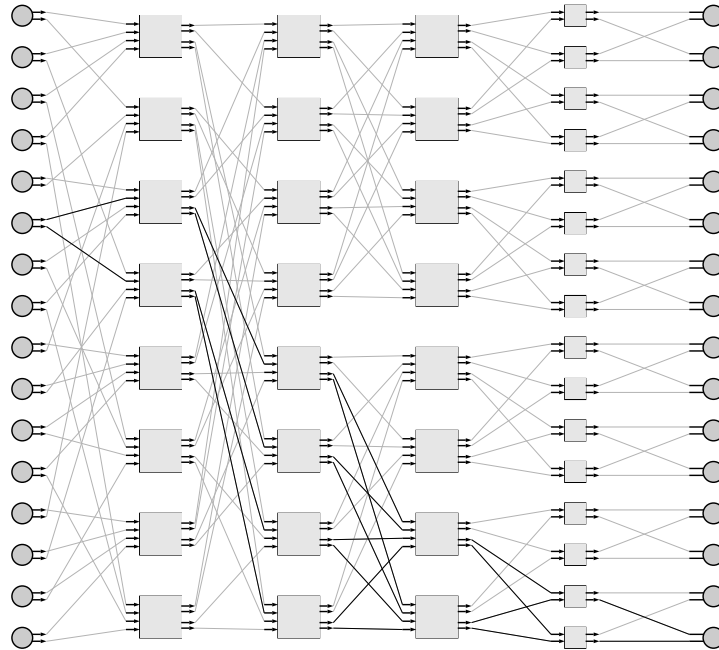
Figure 20.7 16 × 16 Square Multipath Network Constructed from 4 × 2 Crossbars with a Dilation of 2
