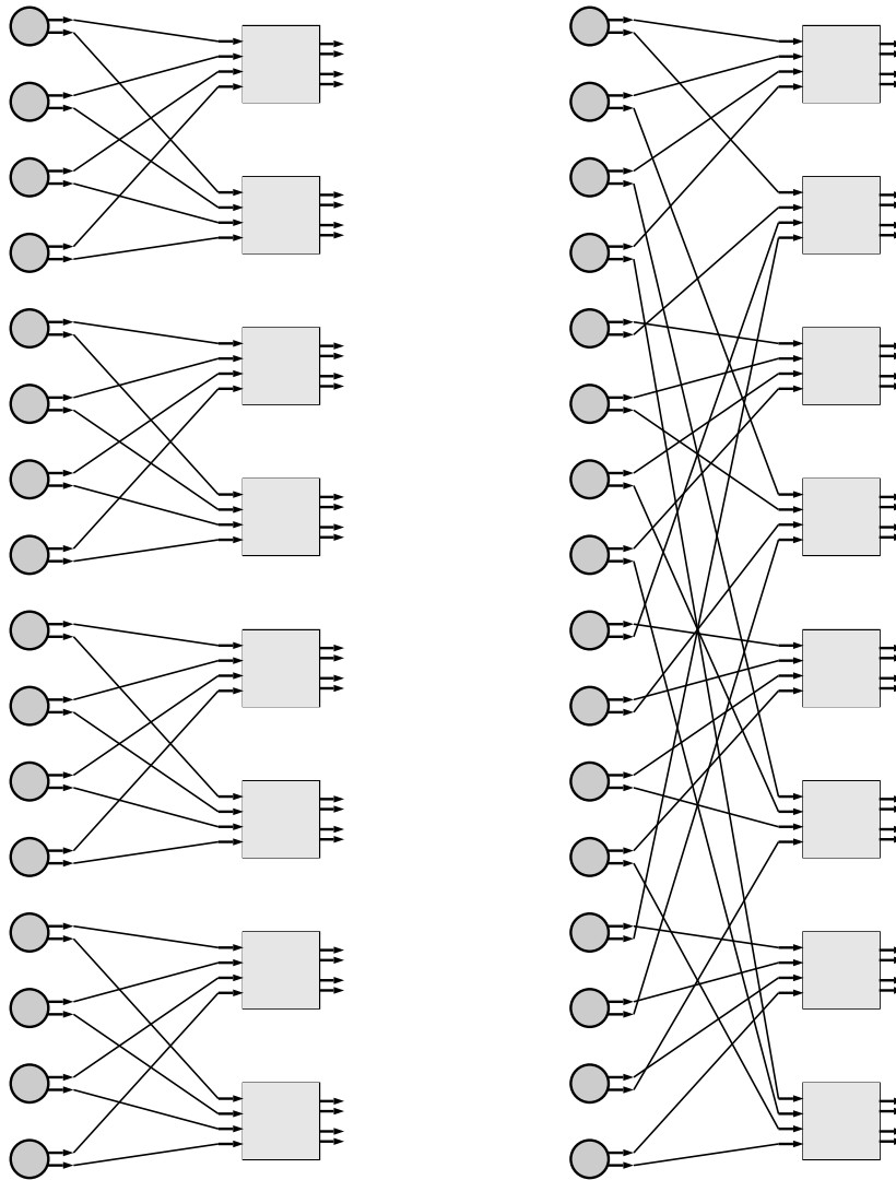
Figure 20.4 Left: Non-expansive Wiring of Processors to First Stage Routing Elements Figure 20.5 Right: Expansive Wiring of Processors to First Stage Routing Elements
