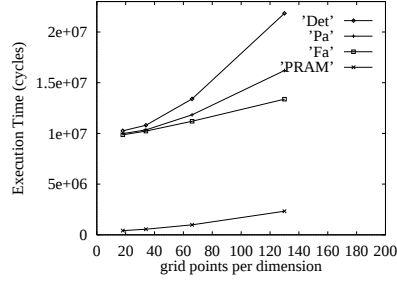
Fig. 1. OCEAN execution time.
