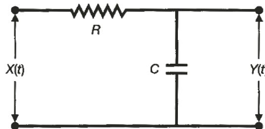
Fig. 6-7 RC filter.
