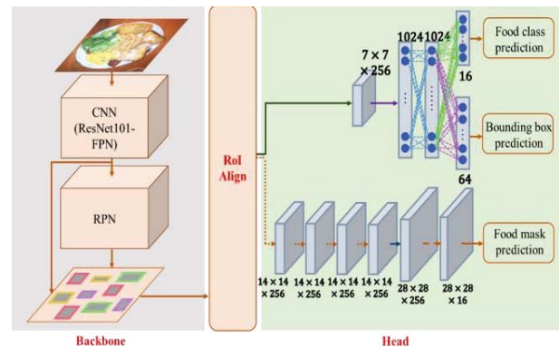
Figure 2. The architecture of mask R-CNN.
